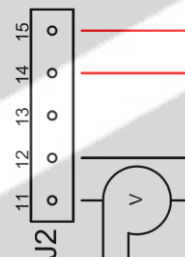
Fig. 8 Wiring diagram for the exclusion of the check of the preheater switch in OIL versions
