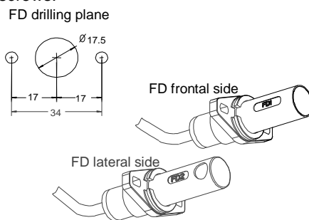
Fig. 4 – Type and fixing systems of FD.. sensors
