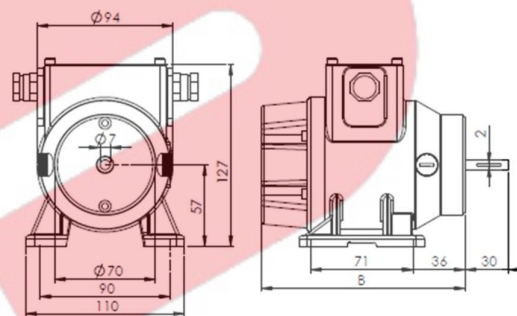
RE.0444R – B3 foot
